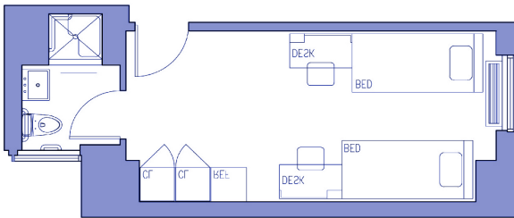
Sample double floor plan
